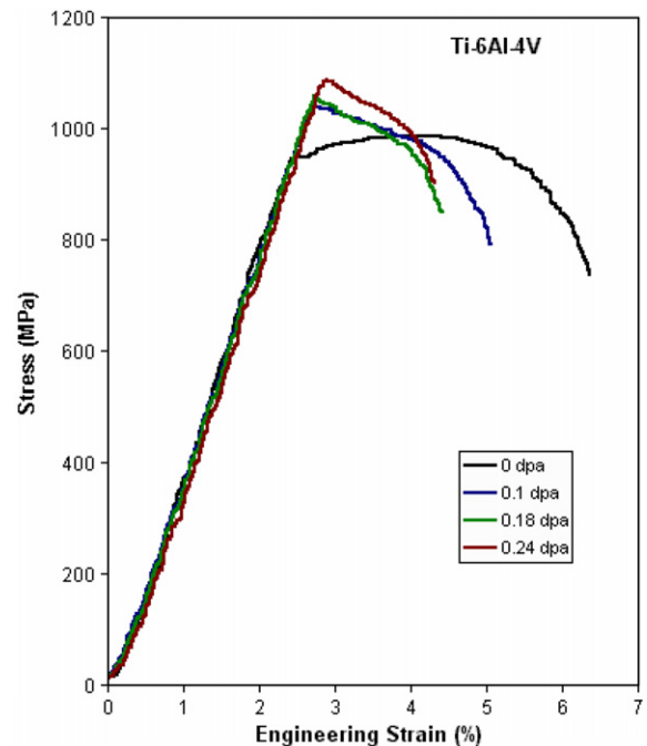
Fig. 13. Irradiation effects on the stress–strain relation of Ti-6Al-4V.
