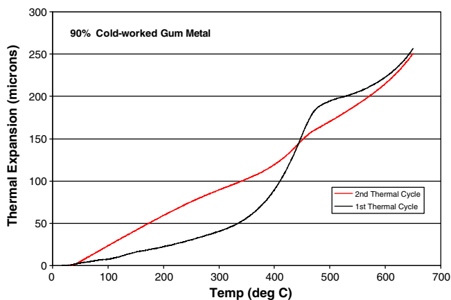
Fig. 18. Effect of temperature on the invar-like properties of the cold-worked ‘gum’ metal shown in Fig. 16(b). Removal of the cold-worked effects that give the alloy invar-like (or very low CTE) behavior below 400 °C and the ‘spike’ in the range of 400–500 °C occurs with a single thermal cycle whose peak temperature exceeds 500 °C.
