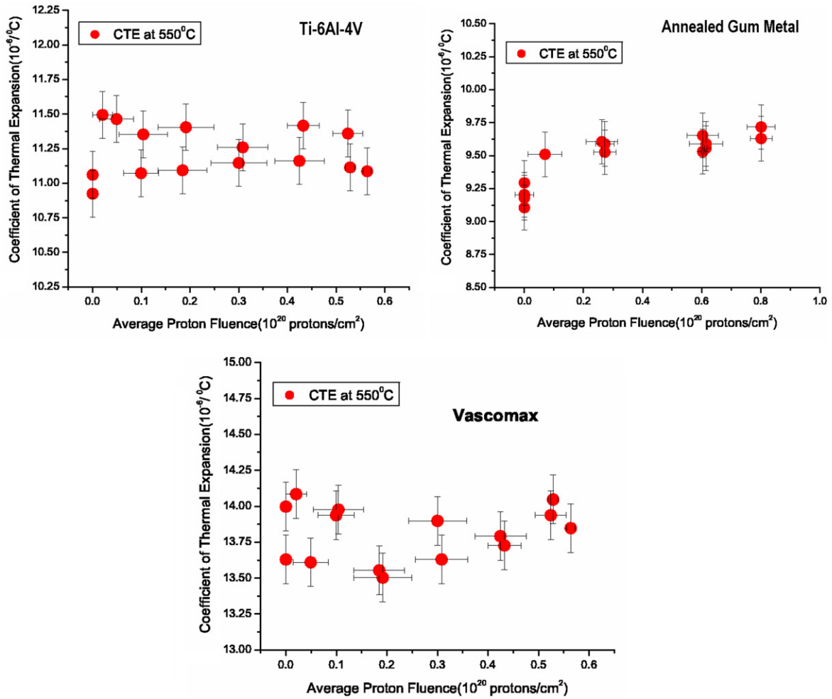
Fig. 11. Irradiation effects on the CTE of several mid-Z materials exposed to protons.
