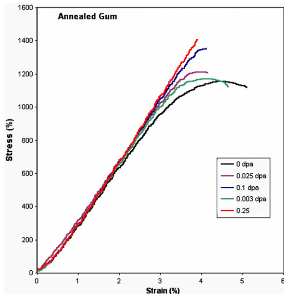
Fig. 17. Irradiation effects on the stress–strain relation of the annealed gum metal. As shown, modest levels of irradiation remove the super-ductility exhibited by the alloy entirely. Note that while the elastic limit and elastic strength of the un-irradiated material (0 dpa) points more towards the cold-worked material, as depicted in Fig. 16, thermal expansion analyses of the un-irradiated samples confirmed that the material tested was much closer to the annealed than to the 90% cold-worked state.
