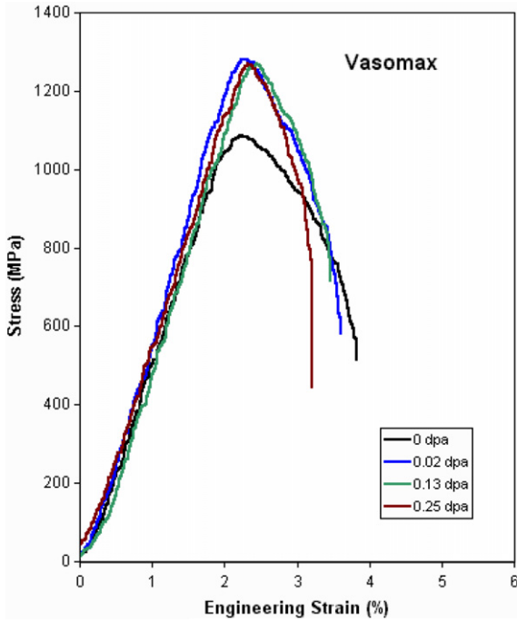
Fig. 14. Irradiation effects on the stress–strain relation of Vascomax-350.
