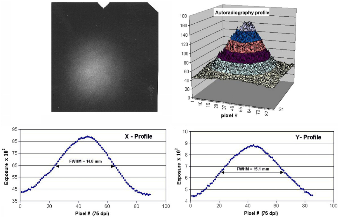
Fig. 5. Autoradiography on embedded nickel films and assessment of proton beam profile.
