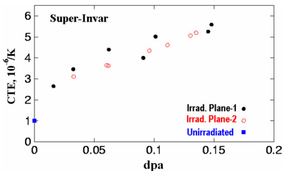
Fig. 7. Effects of modest levels of irradiation damage on the thermal expansion coefficient (CTE) of super-invar.
