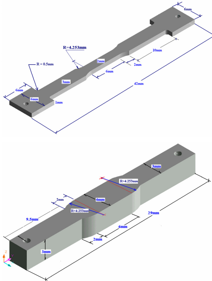
Fig. 3. Specimen design for mechanical and physical property studies.
