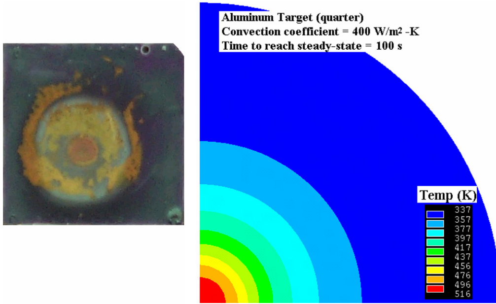
Fig. 4. Irradiation temperature assessment during BNL BLIP operations. On the left the actual target 'painted' with thermal sensitive paint (TSP) is shown following exposure to the beam and after reaching steady-state conditions. On the right are simulation results that helped benchmark the thermo-hydraulic parameters associated with the actual target irradiation set-up.
