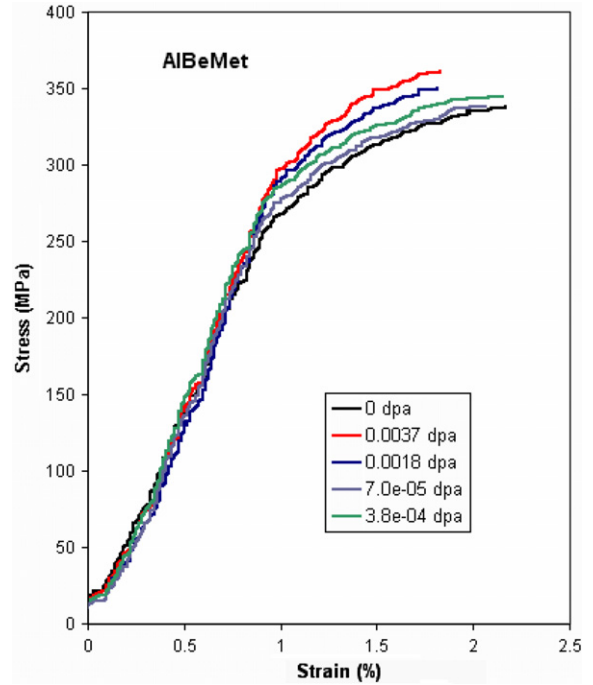
Fig. 15. : Irradiation effects on the stress–strain relation of the low-Z alloy AlBeMet (62% beryllium and 38% aluminum). Noteworthy is the retention of ductility exhibited by the alloy.
