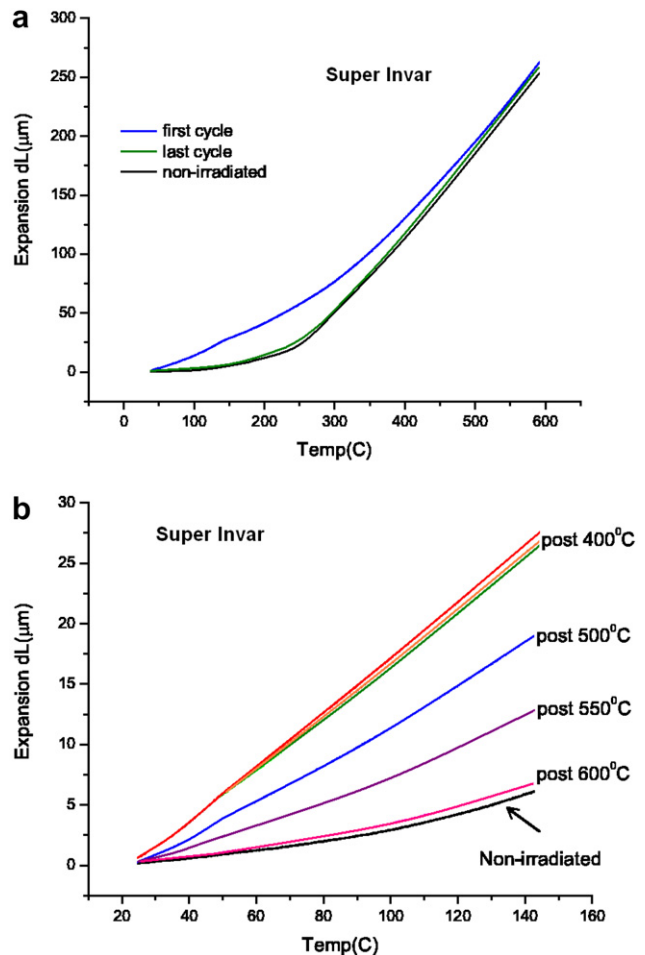
Fig. 9. Effects of post-irradiation ‘annealing’ on super-invar. Thermal cycling with temperatures <400 °C appear to have no effect towards reversing ‘damage’ induced by protons. Thermal cycling with temperatures >600 °C reverse the ‘damage’ entirely.
