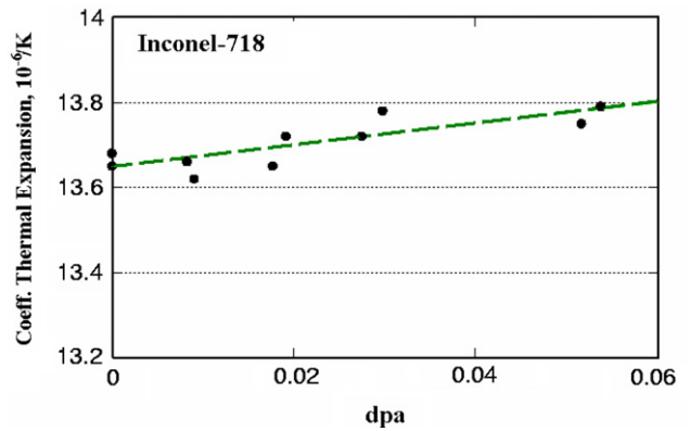
Fig. 8. Proton irradiation effects on the CTE of Inconel-718. The very low dpa associated with inconel-718 is the result of its positioning near the edges of the irradiated plane.
