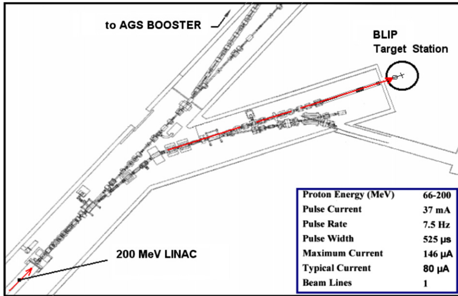
Fig. 1. BNL experimental facilities used in the material irradiation study.
