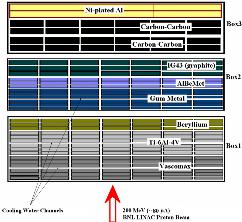
Fig. 2. Specimen layout in the irradiation boxes used the BNL Phase II irradiation.
