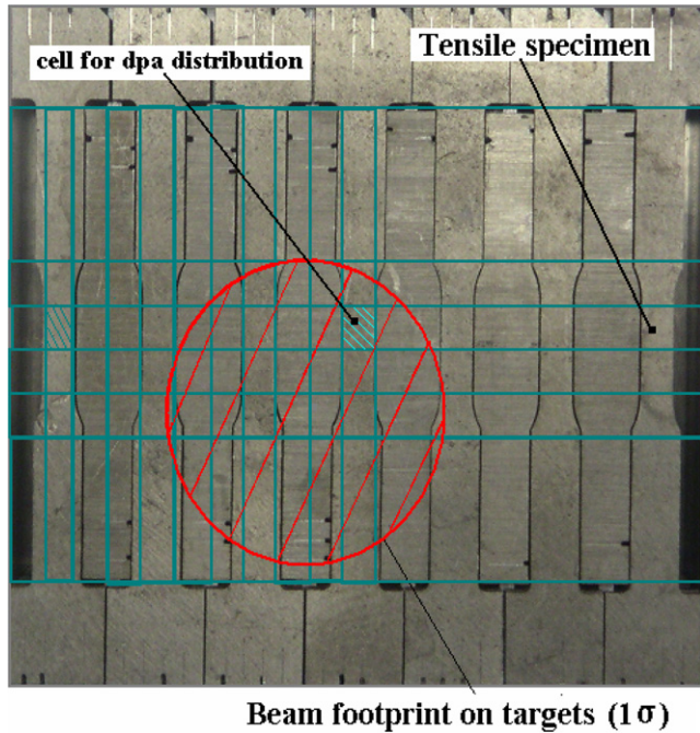
Fig. 6. Integration of different types of specimens into the irradiation space. Also shown is the special numbering of the specimens used. Superimposed is the approximate location of the beam footprint and the discretization used for the spatial distribution of irradiation damage.
