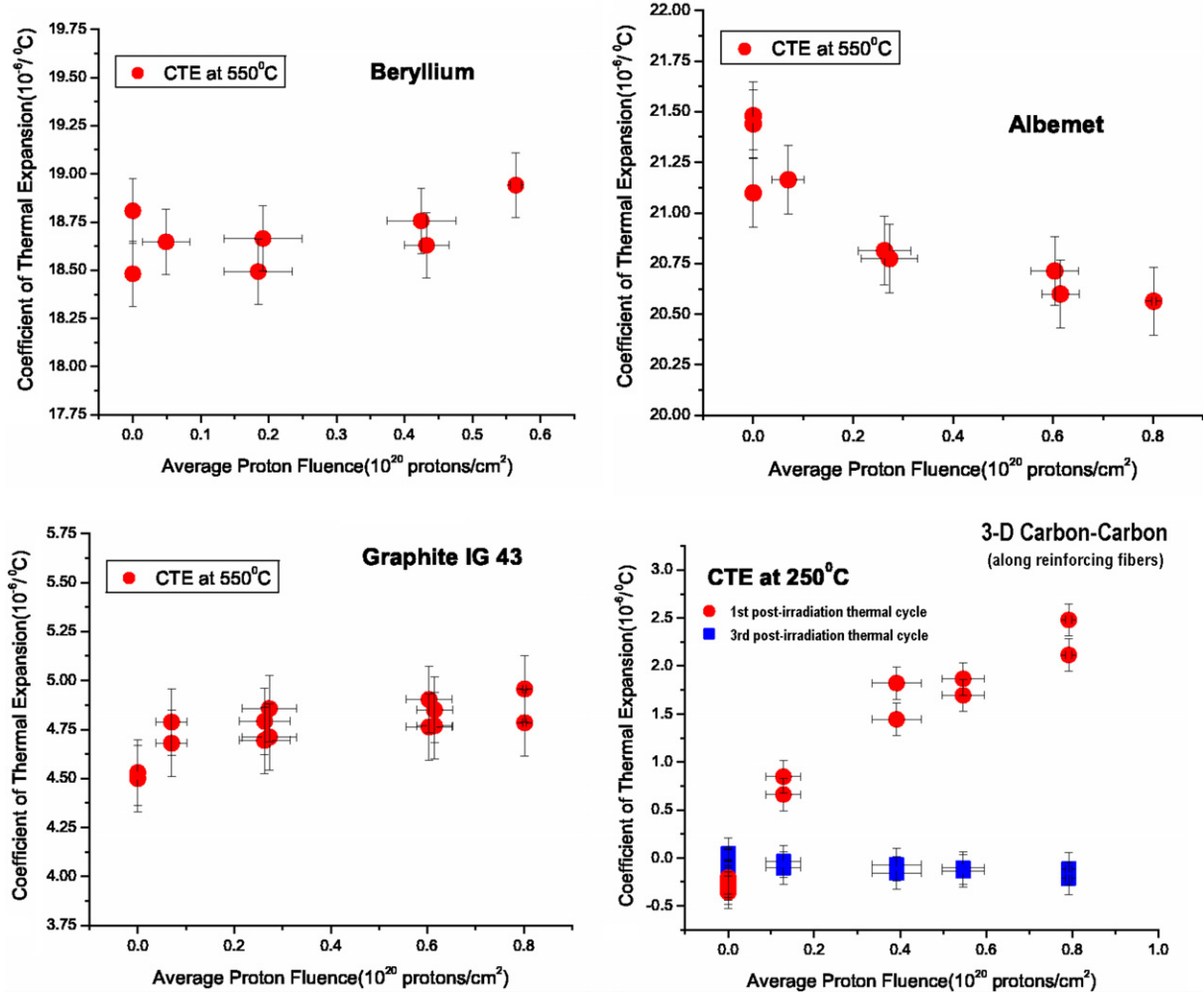
Fig. 10. Irradiation effects on the CTE of several low-Z materials exposed to protons. The dramatic effects of irradiation on the CTE of the 3D carbon composite and of the post-irradiation annealing through thermal cycling are evident in (d). Similar ‘annealing’ behavior was observed in the 2D carbon composite along the strong (fiber-reinforced) and the ‘weak’ (normal to fiber planes) directions.
