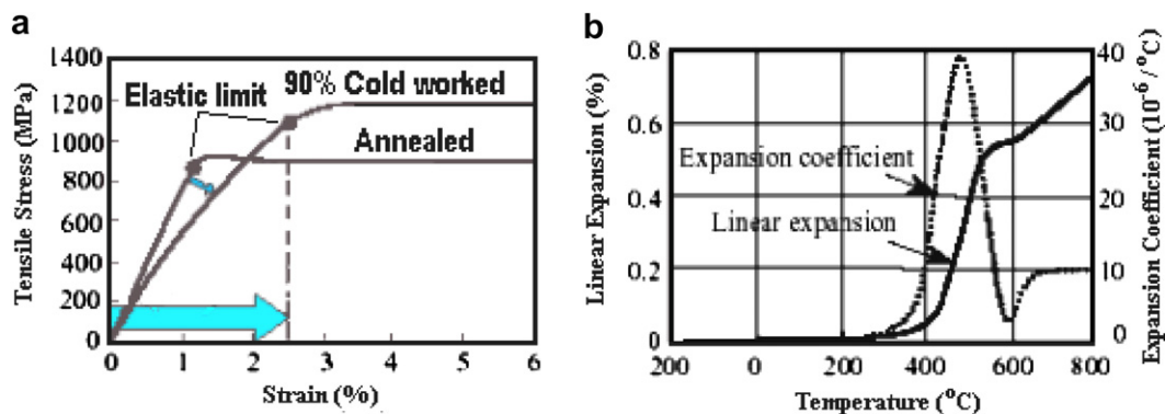
Fig. 16. Mechanical and thermal properties of the super alloy ‘gum’ metal [7]. (a) Depicts the stress–strain relation of the annealed and cold-worked forms of the alloy. (b) Shows the thermal expansion and CTE of the cold-worked ‘gum’ metal.
