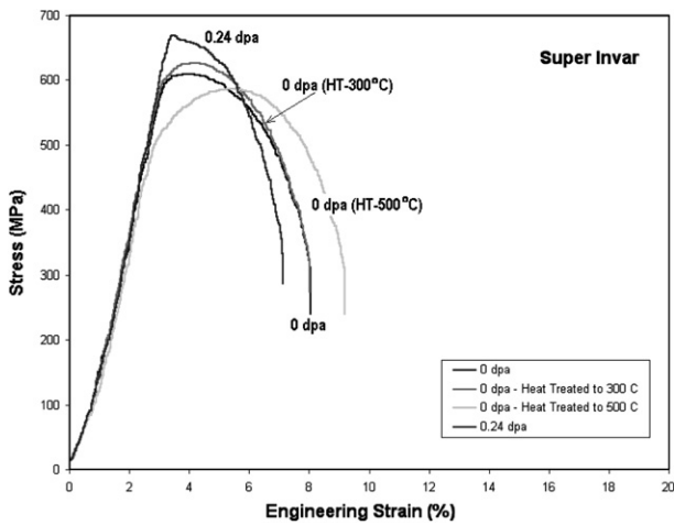
Fig. 12. Irradiation and heat treatment effects on the stress–strain relation of super-invar.
